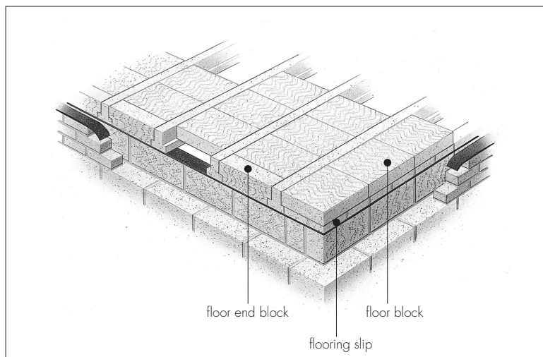
Figure 1 Typical floor arrangement
